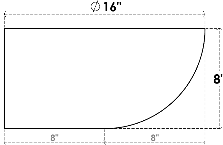
SIDE PROFILE
